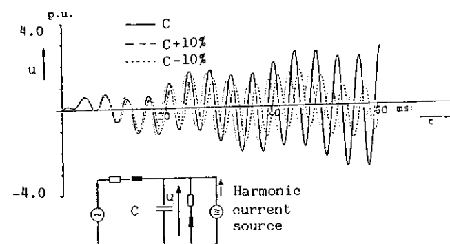
b) Resonance phenomena, variation of capacitances
