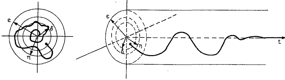
Figure 2. Illustration of the definition of asymptotic stability [25].
