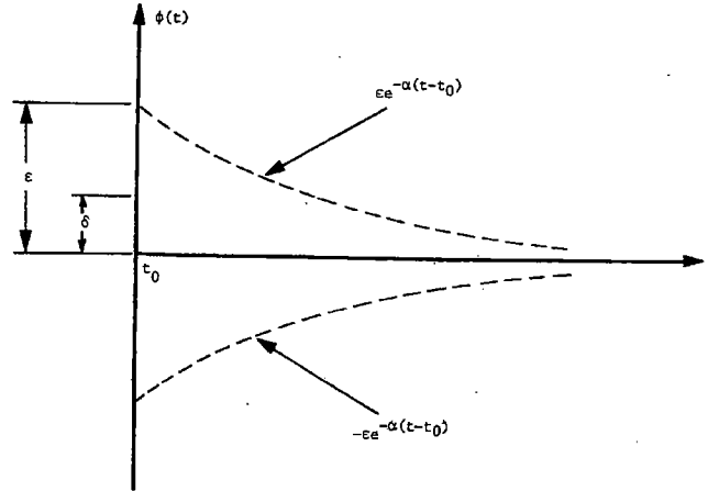
Figure 4. Illustration of the definition of exponential stability [26].
