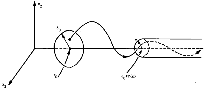
Figure 3. Illustration of the definition of uniform asymptotic stability [26].
