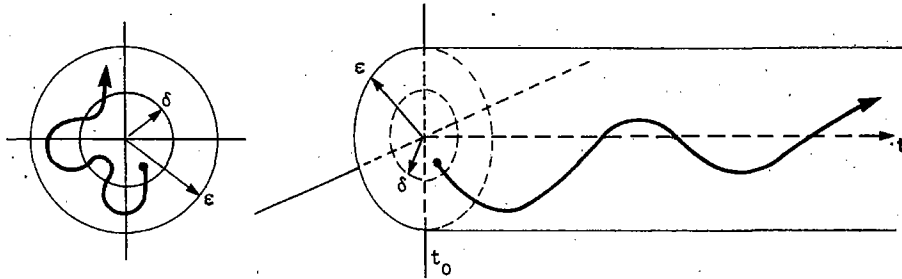
Figure 1. Illustration of the definition of stability [25].
