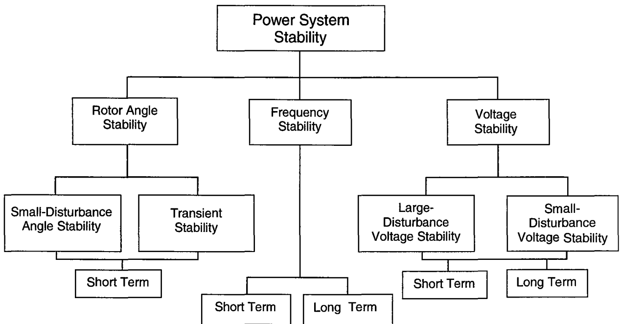
Figure 5. Classification of Power System Stability
