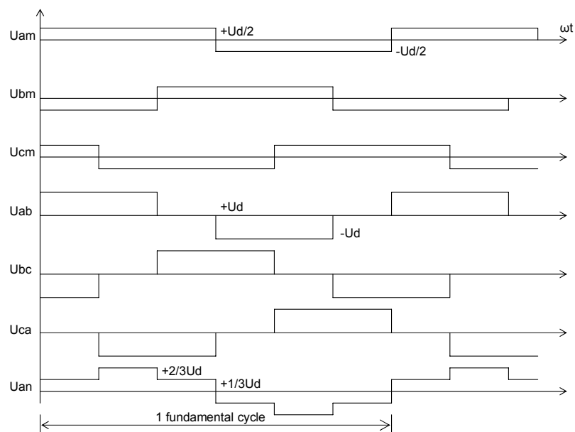
Figure 3.5: VSC voltages converter side—square wave operation
