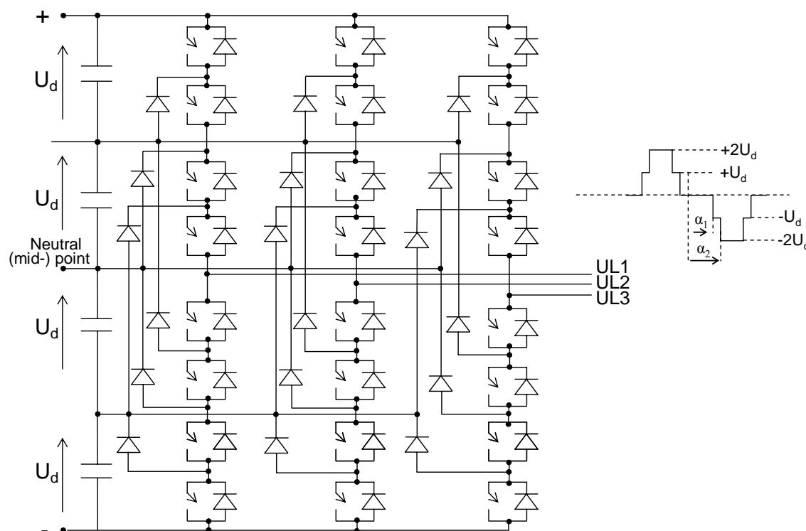
Figure 4.5: Three-phase 5-level NPC converter and associated ac voltage waveform for one phase
