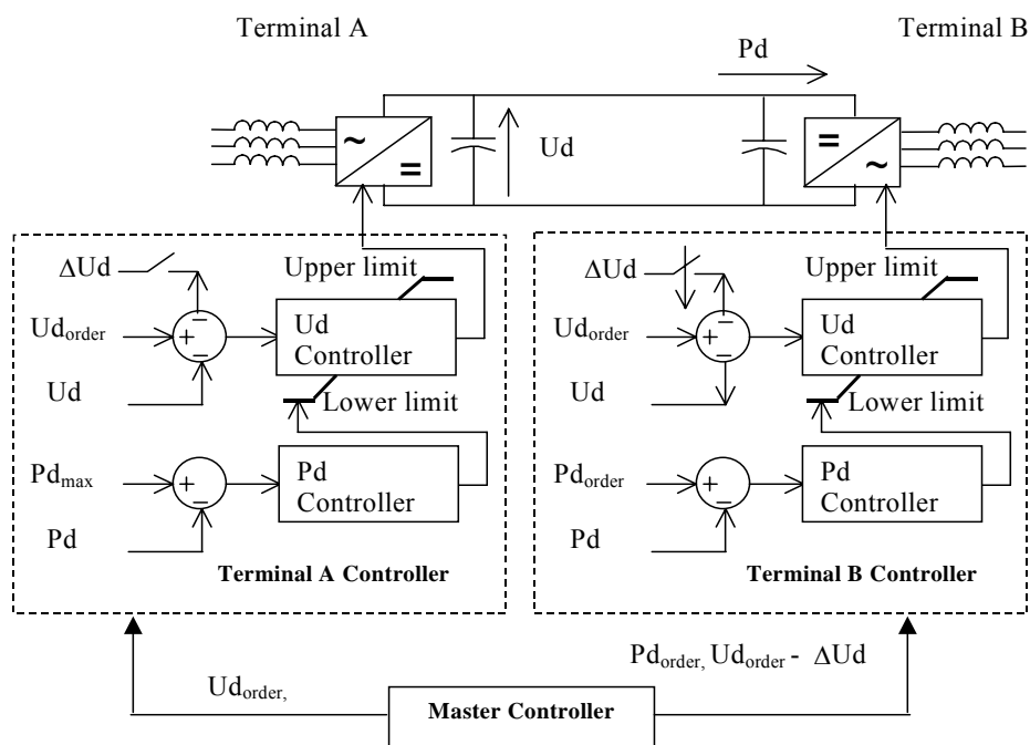
Figure 7.9: Coordination control example for two-terminal VSC Transmission
