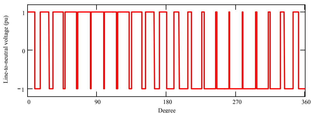
Figure 4.2: Single-phase ac voltage output for 2-level converter with PWM switching at 21 times fundamental frequency
