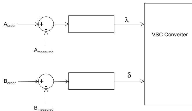
Figure 7.2: Direct control of Modulation Index \lambda and phase angle \delta by parameters A and B
