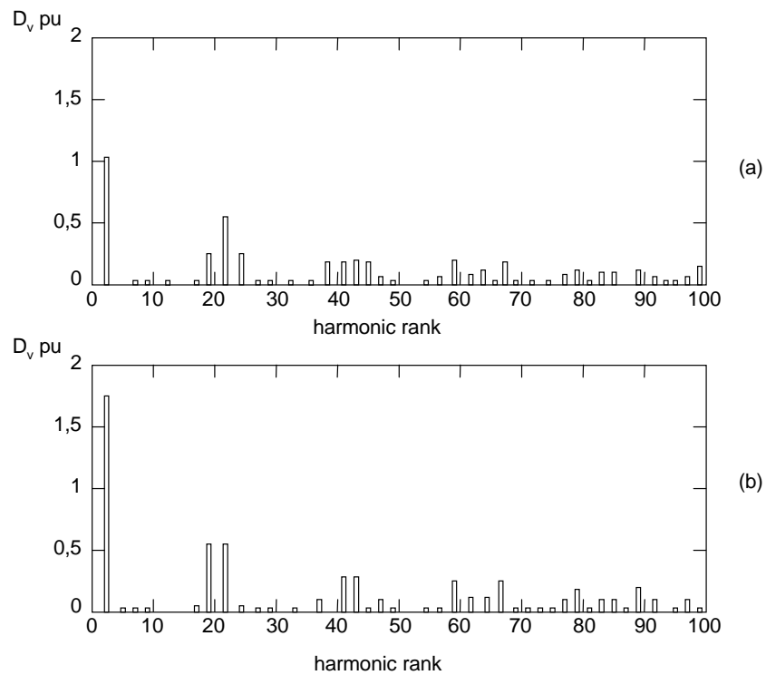
Figure 9.3 Voltage harmonics spectra of a 2-level VSC with carrier frequency at 21 st harmonic
