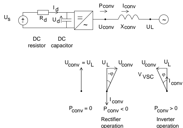
Figure 2.2: The principle of active power control
