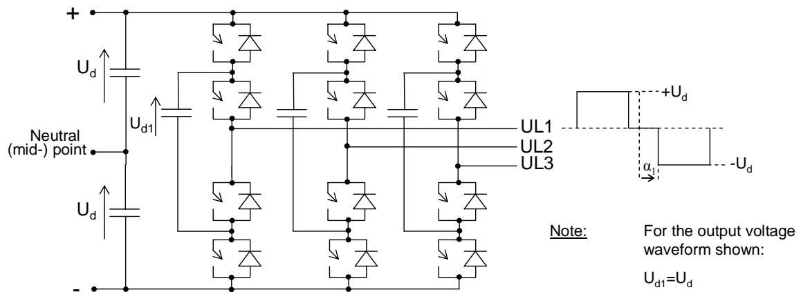
Figure 4.6: Diagram of a three-phase 3-level floating capacitor converter and the associated ac voltage waveform for one phase
