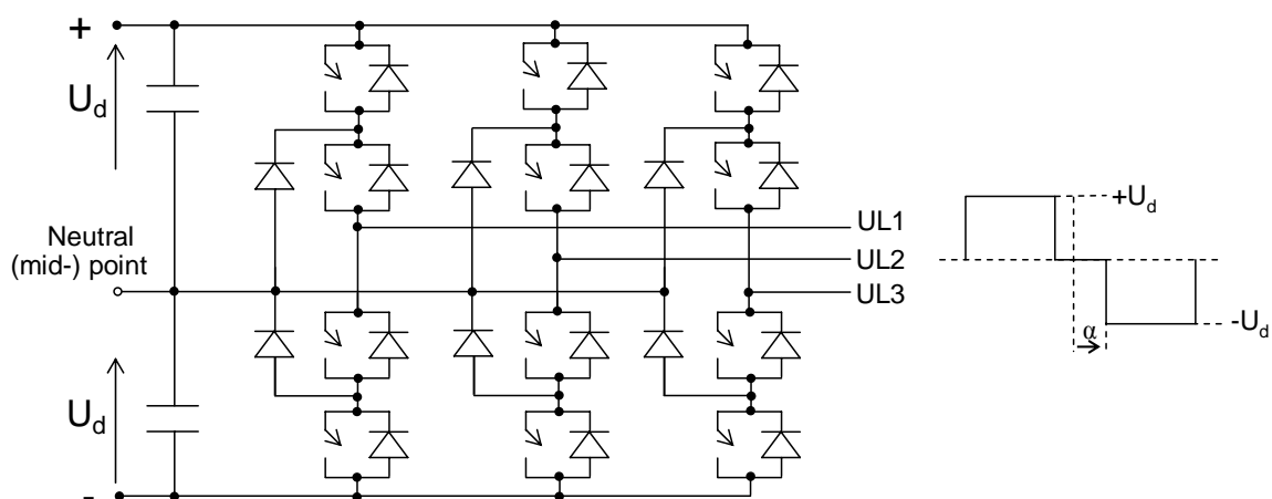
Figure 4.3: Three-phase 3-level NPC converter and associated ac voltage waveform for one phase
