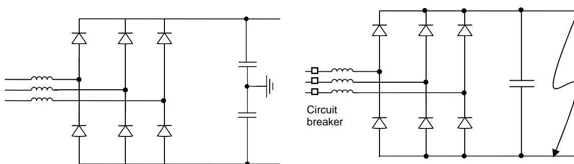
Figure 5.3: A 2-level VSC bridge with the IGBTs turned off
