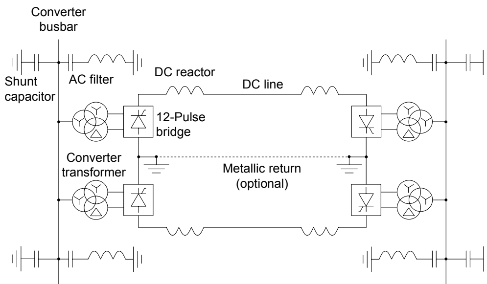
Figure C.1: One-line diagram of a two-terminal HVDC system
