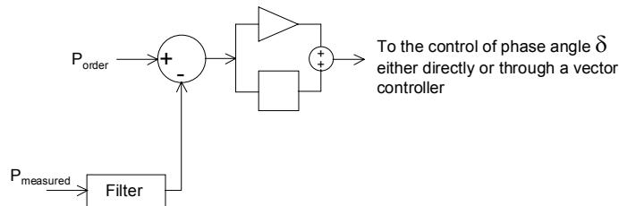
Figure 7.5: VSC power controller
