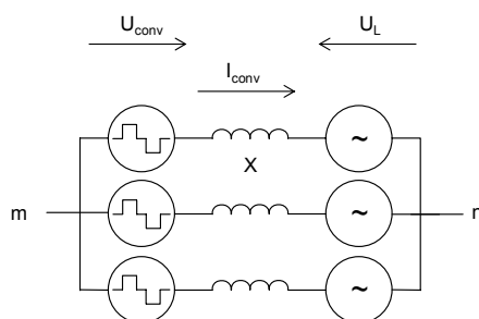
Figure 3.6: Equivalent circuit VSC
