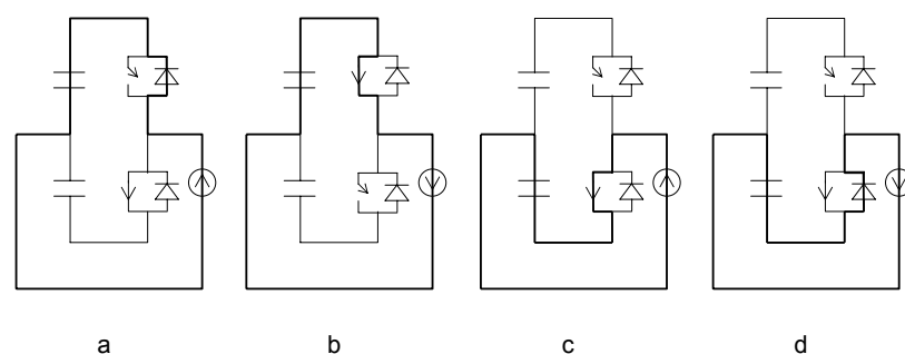
Figure 3.3: The four possible current paths in a single-phase, 2-level VSC
