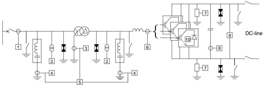
Figure 8.1: Protection concept of a VSC substation
