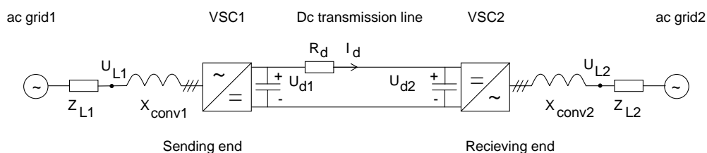
Figure 2.5: A point-to-point VSC Transmission scheme
