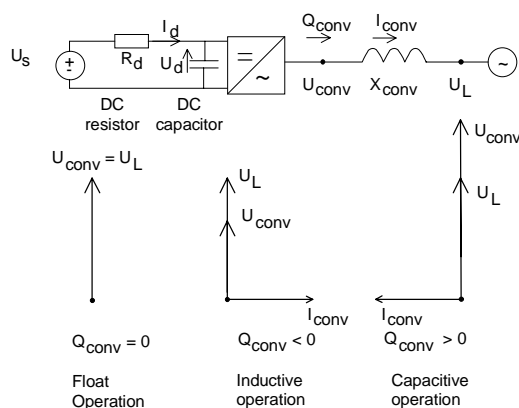
Figure 2.3: The principle of reactive power control
