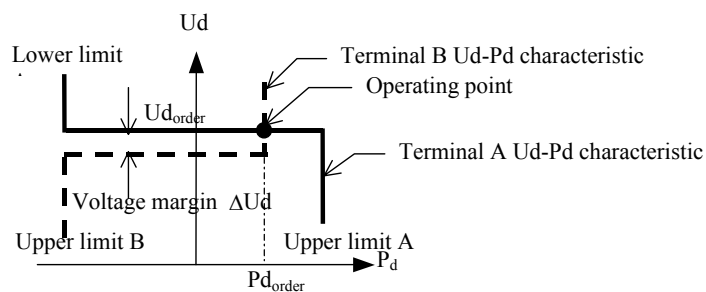
Figure 7.10: Operating point in voltage margin method
