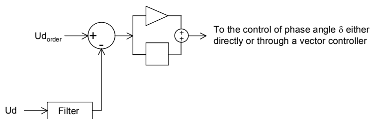
Figure 7.6: DC voltage controller
