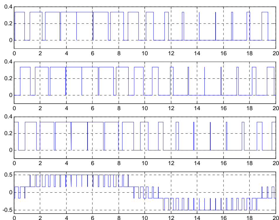
Figure 9.5: Voltage generated by one phase unit, 4 levels VSC voltage (y axis, pu) versus time (x axis, ms). From upper to lower window:
