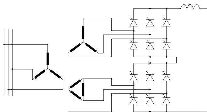
Figure C.2: Configuration of a 12-pulse bridge
