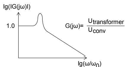
Figure 6.4: Typical magnitude-frequency-characteristic of an HF blocking filter
