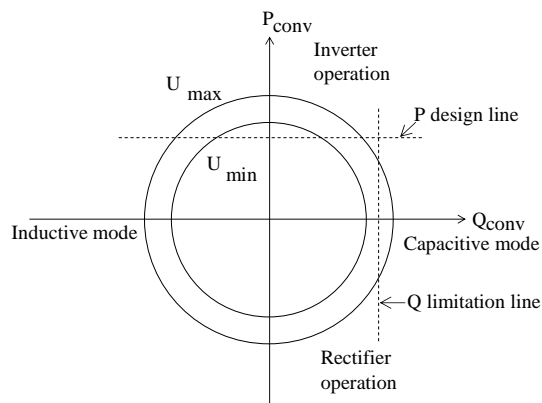
Figure 2.4: A basic simplified PQ diagram
