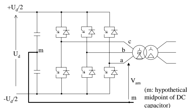
Figure 9.1: 2-level VSC
