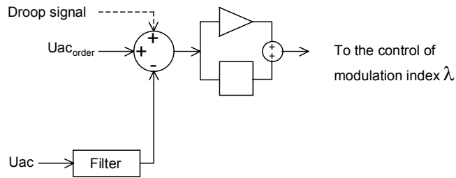
Figure 7.4: AC voltage controller
