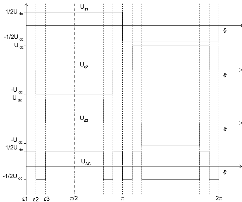
Figure 9.4: Graphical explanation of the SHEM principle (5 th harmonic elimination)
