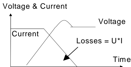
Figure 5.5: Voltage and current across an IGBT and diode during switching
