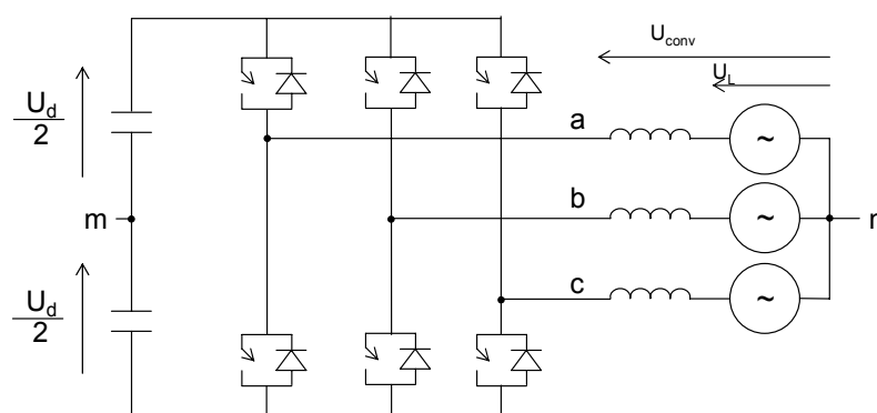
Figure 3.4: The basic 2-level, 6-pulse VSC—three-phase configuration
