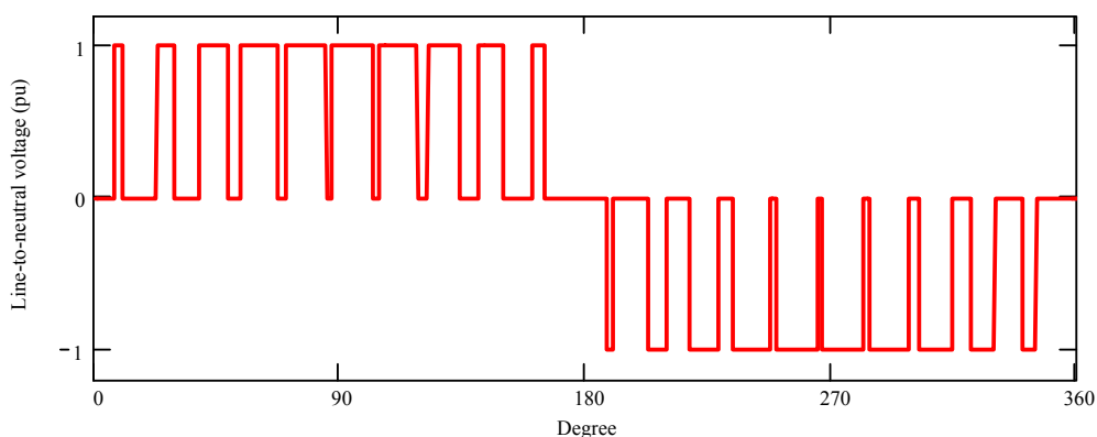
Figure 4.4 Single-phase ac voltage output for 3-level NPC converter with PWM switching at 21 times fundamental frequency
