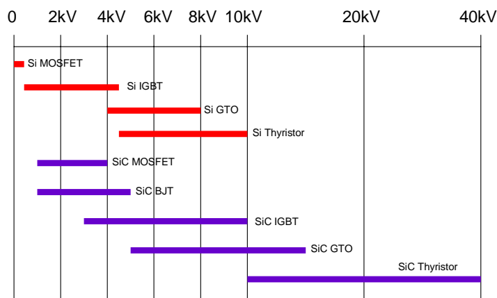
Figure 15.2: Silicon carbide (SiC) switches compared to silicon (Si) switches
