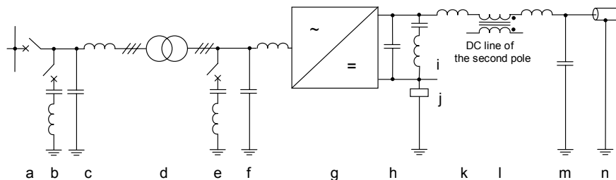
Figure 6.1: Major components that may be found in a VSC substation
