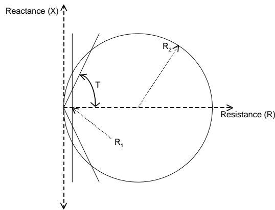
Figure 9.8: Boundaries of harmonic impedance loci at the POC
