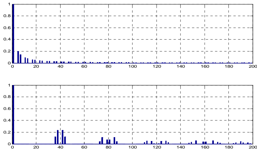
Figure 9.6: Spectrum of phase-to-phase voltage at a 2-level phase unit output, amplitude (y axis, pu U 1 based) versus harmonic rank (x axis, 50-Hz based) - Upper graph: Full wave modulation - Lower graph: Carrier-modulated method at 2kHz
