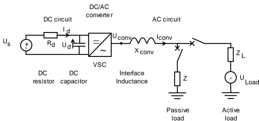
Figure 2.1: Diagram of a generic voltage sourced converter
