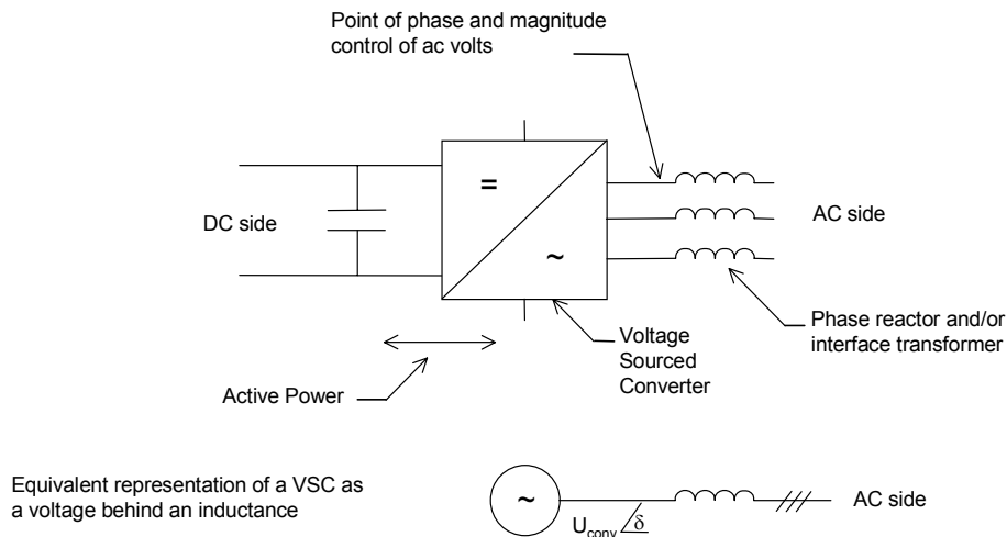
Figure 7.1: Representing a VSC unit as an ac voltage magnitude U and angle \theta behind reactance
