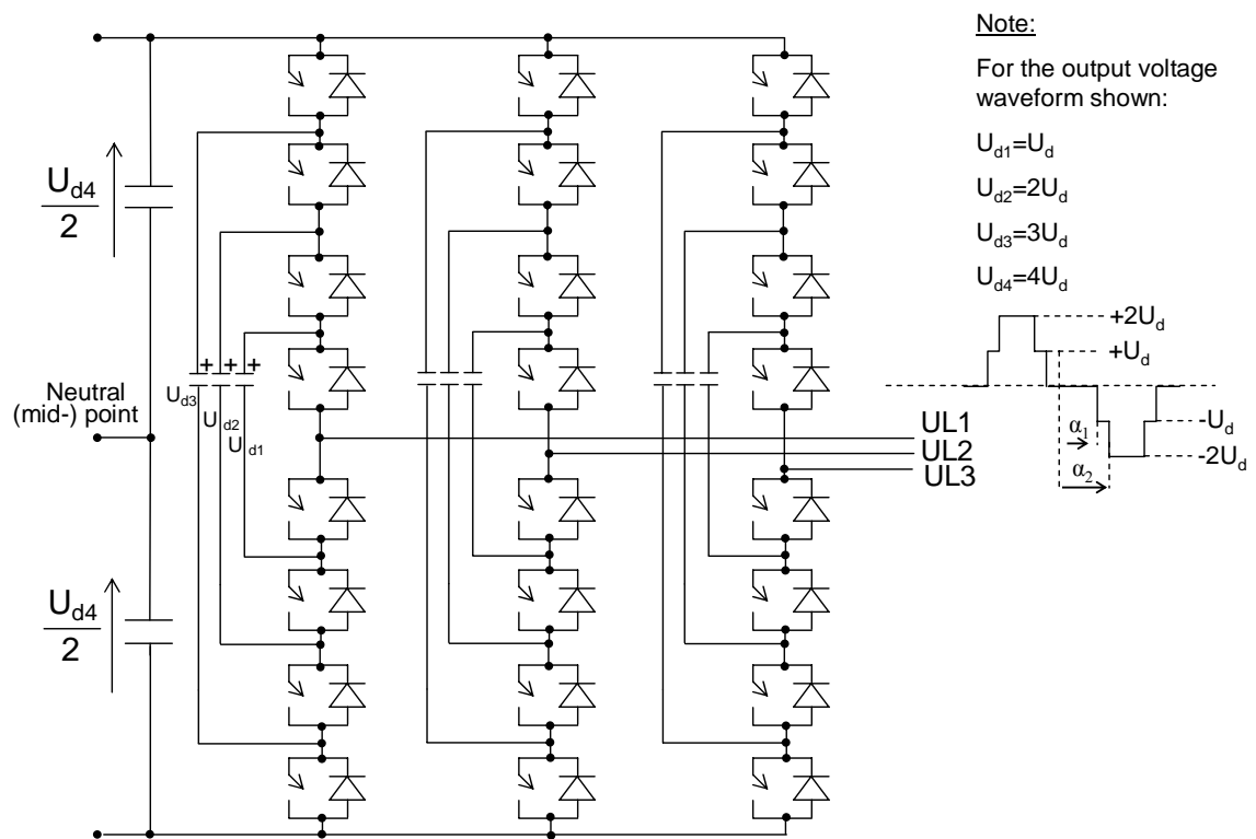
Figure 4.7: Three-phase 5-level floating capacitor converter and associated ac voltage for one phase
