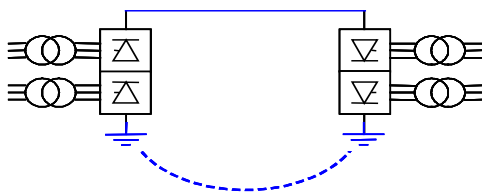
Figure 3.2.a Ground Return
