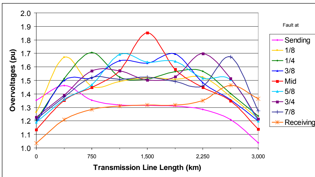
Figure 4.8: 3,000 km Transmission Line.
