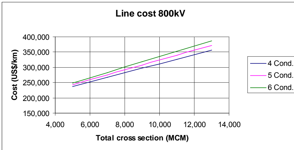
Figure 4.33: Line Costs \pm 800 kV
