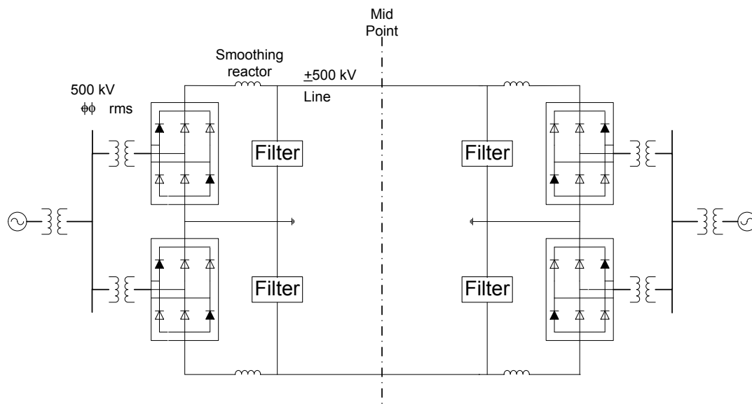
Figure 4.1: HVDC system modeling for fault application calculation
