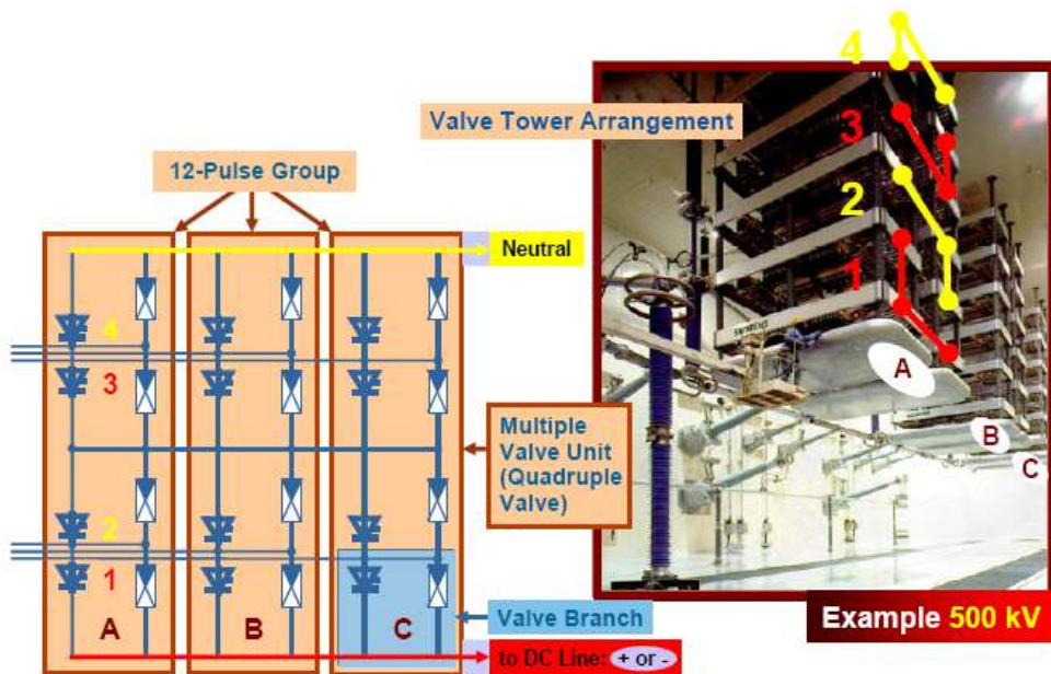
Figure 5.11: Example of a \pm 500 kV 12-Pulses Valve Tower Configuration
