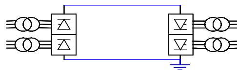
Figure 3.2.b Metallic Return
