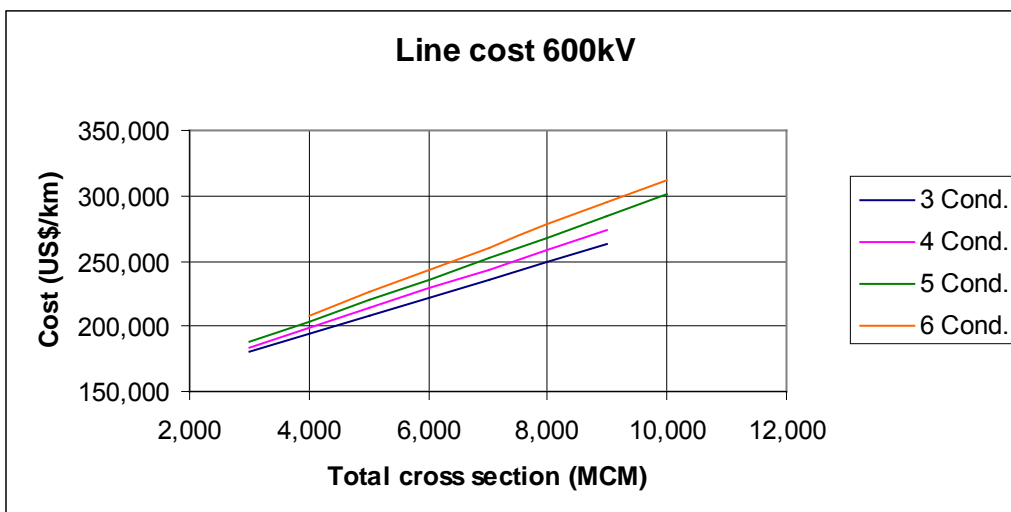
Figure 4.32: Line Costs \pm 600 kV
