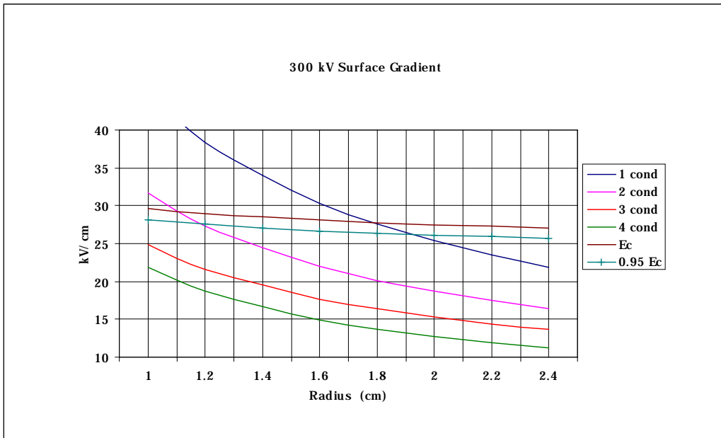
Figure 4.19: Conductor Surface Gradients \pm 300 kV
