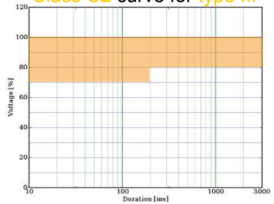
Class C2 curve for type III
