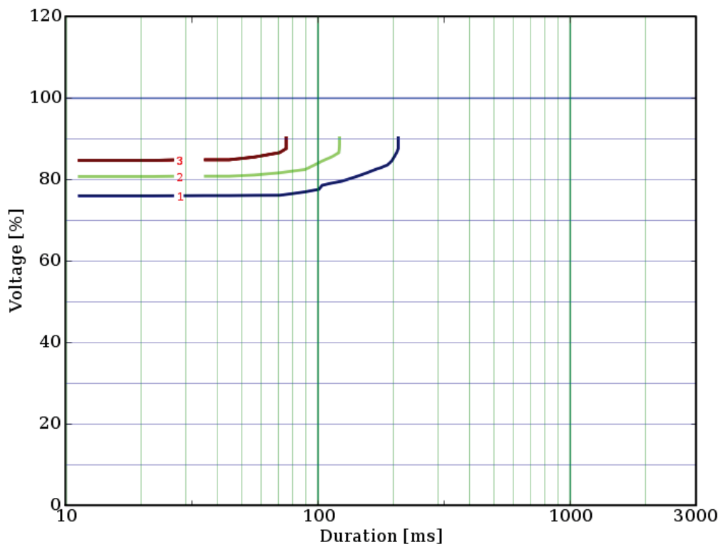
Figure 6-28 MV and HV sites, "MANY" scope (3 voltage channels recorded), type I and (3B) shape at the same time, 75% best sites.
