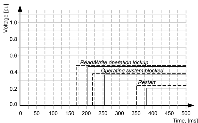
Figure 3-22 Voltage-tolerance curves for PC with switched-mode power supply: three different malfunction criteria and two different supply voltages (230V/50 Hz, solid line, and 110V/60Hz, dashed line) [29].
