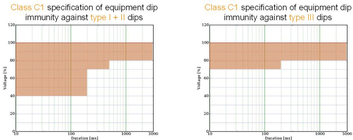
Figure 7-3 Voltage-tolerance curves for Class C1 specification of equipment dip immunity.
