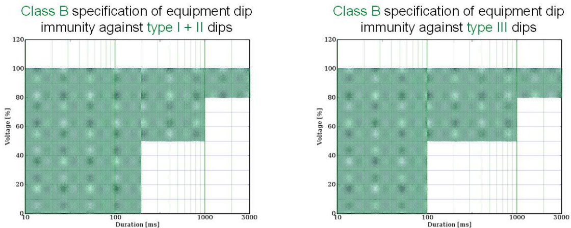
Figure 7-2 Voltage-tolerance curves for Class B specification of equipment dip immunity.
