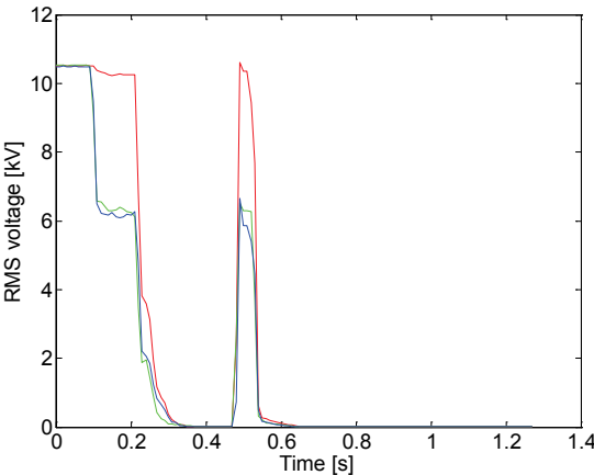
Figure 2-11 Multiple short interruption event caused by a fault and unsuccessful autoreclosing.
