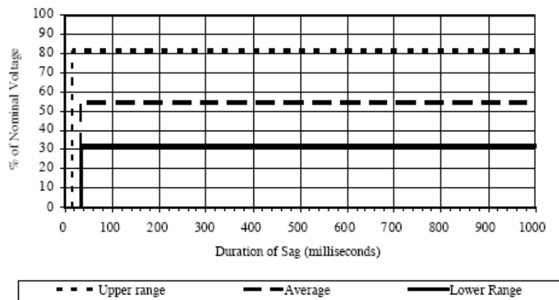
Figure 3-21 PLC ac input card voltage tolerance curves [28].
