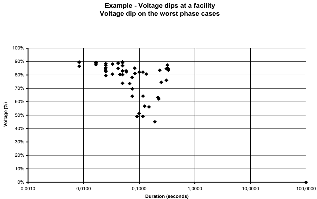
Figure 7-9 Voltage dips recorded at an end-user facility over a 1.5 year period.
