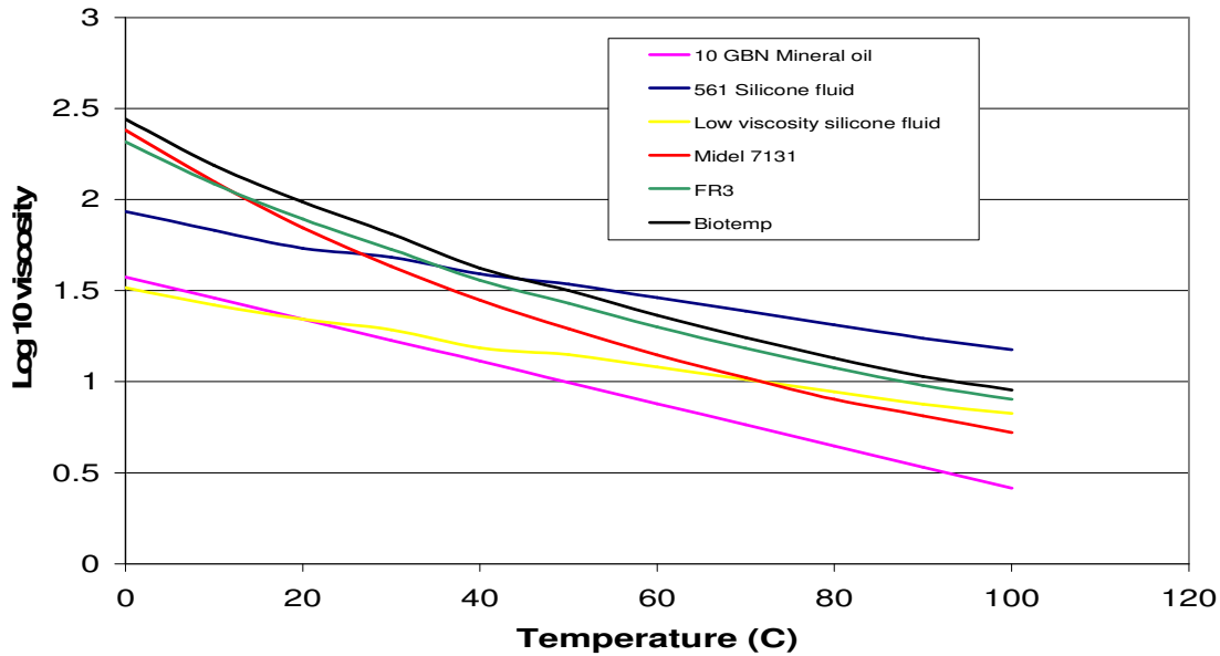
Figure 3.5 – Log 10 (viscosity) vs temperature
