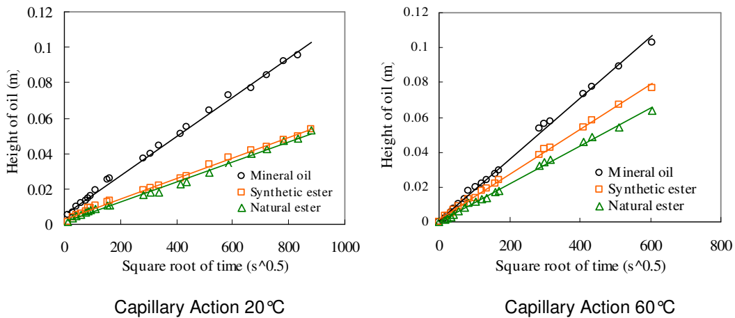
Figure 9.2 – Graphs of Capillary action at 20°C and 60°C
