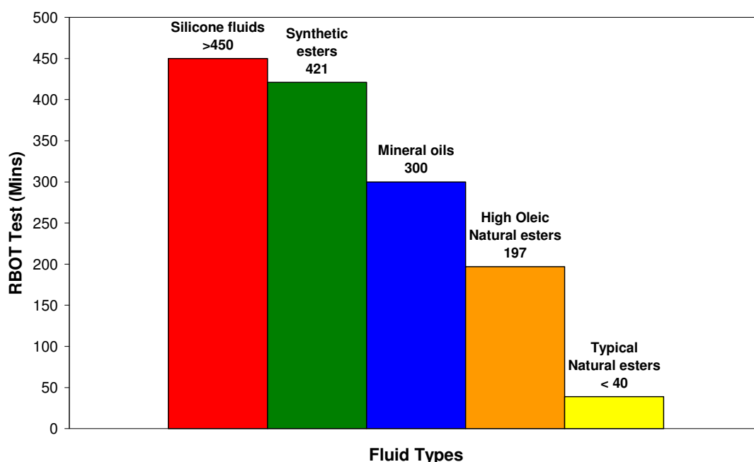
Figure 3.12 – RBOT test results for different dielectric fluid types
