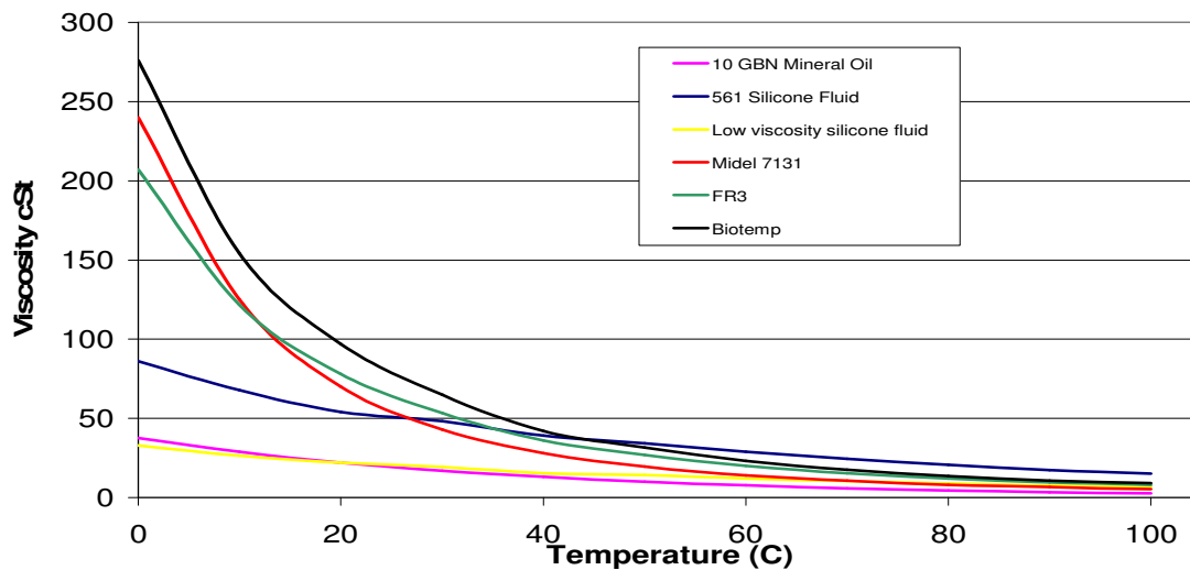
Figure 3.6 – Comparative viscosities with varying temperature
