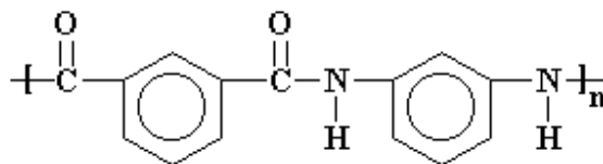
Figure 9.6 - Nomex - Meta linked aramid
