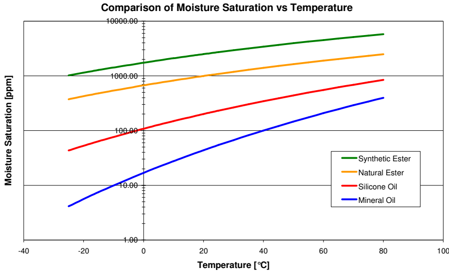
Figure 3.8 – How moisture saturation varies with temperature
