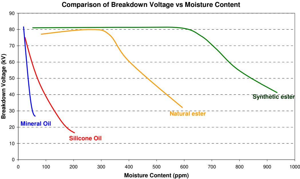
Figure 4.1 – Effect of absolute moisture content on AC breakdown strength of clean fluids
