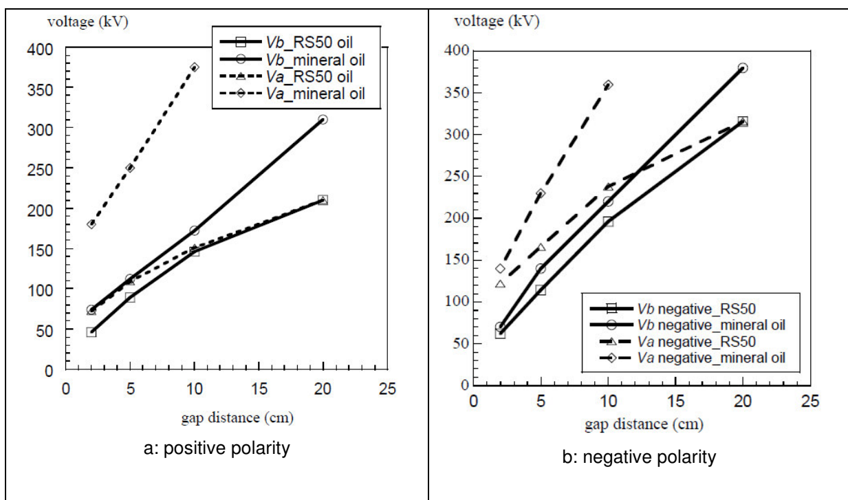
Figure 4.8: Breakdown voltage ( V_b , 50% probability) and acceleration voltages ( V_a ) for positive (a) and negative (b) voltages for mineral oil and a specific rape-seed based liquid. (Point-to-plane gap, fast rise time/long tail impulse) 65
