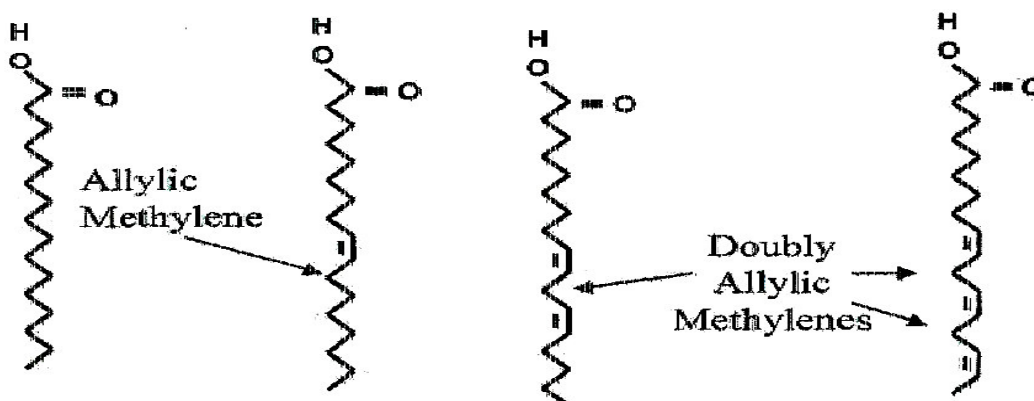
Figure 3.11 - Types of unsaturation found in natural ester fatty acid chains (Source: CARGILL)
