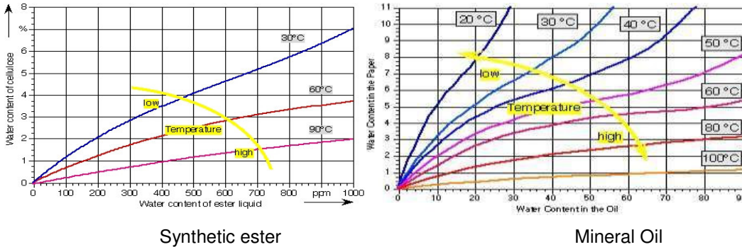
Figure 9.4 – Graphs of Moisture equilibrium in synthetic ester and mineral oil
