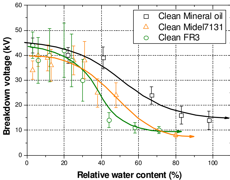
Figure 4.3 – Effect of relative moisture content on AC breakdown strength of clean fluids
