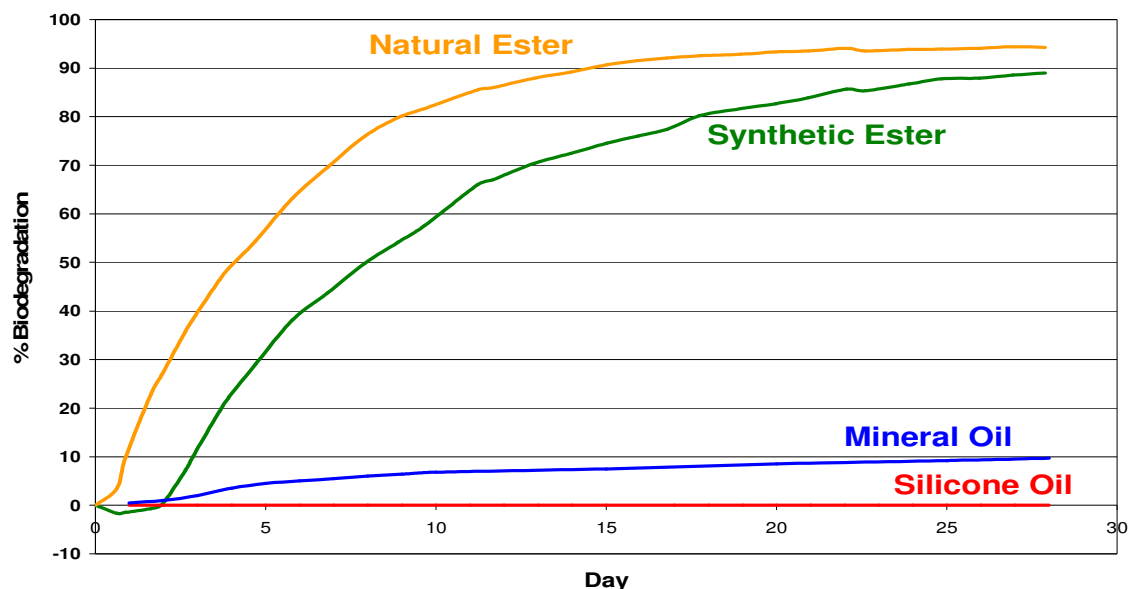
Figure 3.9 - Comparison of biodegradation rates
