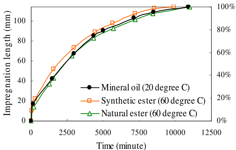
Figure 9.3 – Graph of Impregnation
