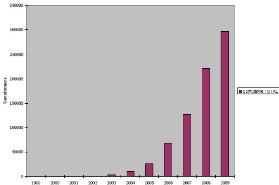
Figure 2.3 - Number of natural ester distribution transformers in service – worldwide
