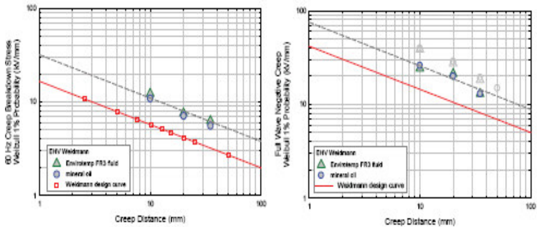
Figure 5.1: 60 Hz and impulse EHV Weidmann creep design curves for natural ester and mineral oil
