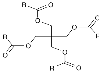
Figure 3.3 – Structure of synthetic ester
