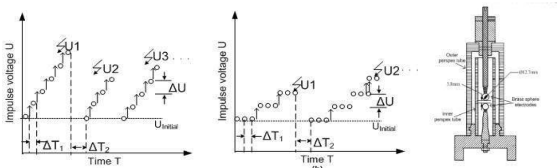
a. 1 shot/step rising-voltage method b. 3shots/step rising-voltage method c. test cell
