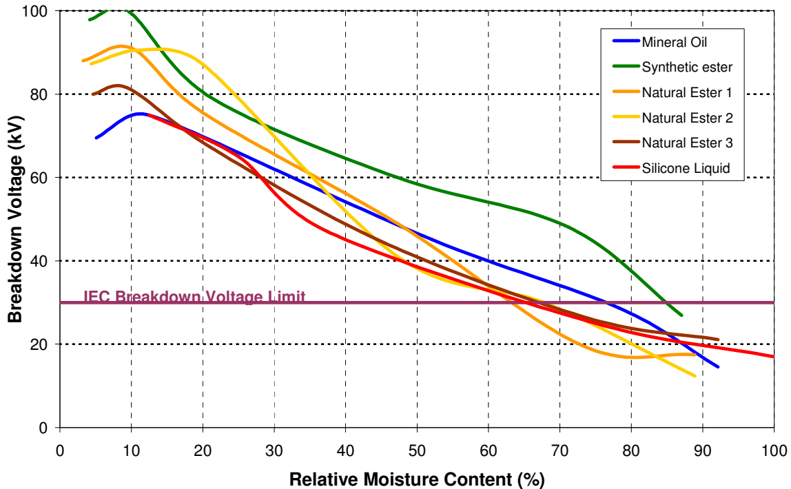
Figure 4.2 – Effect of relative moisture content on AC breakdown strength of fluids
