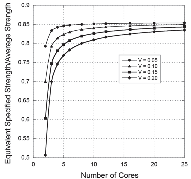
Fig. 4.1.3.2—Ratio of equivalent specified strength to average in-place compressive strength as a function of the number of cores and coefficient of variation of core strengths based on ACI 562.
