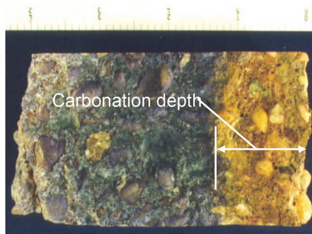
Fig. 4.1.2.2—Depth of carbonation as indicated by color change using a pH indicator solution.
