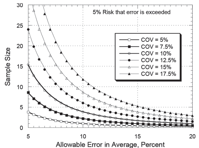
Fig. 4.1.1—Sample size based on ASTM E122; risk = 5 percent.
