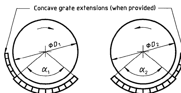
Figure 2 — Longitudinally disposed cylinders or rotors (viewed from rear)
